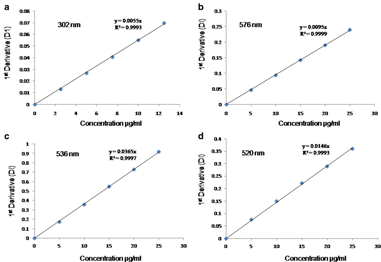
Fig. 2. Linear curve of 1st-order derivative spectra of standard a acetaminophen, b carmoisine, c erythrosine, and d sunset yellow
